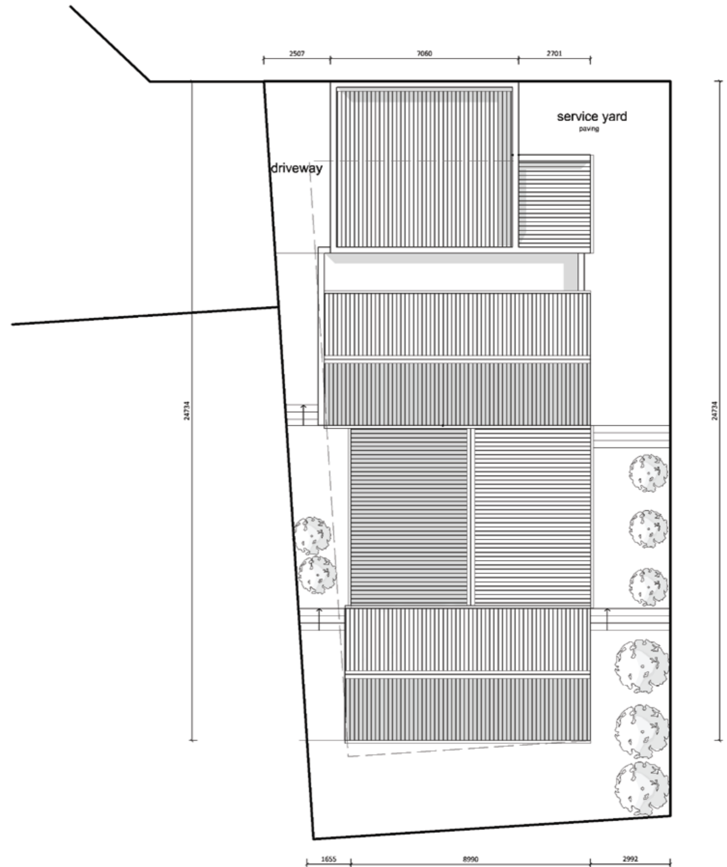
SITE ROOF PLAN
