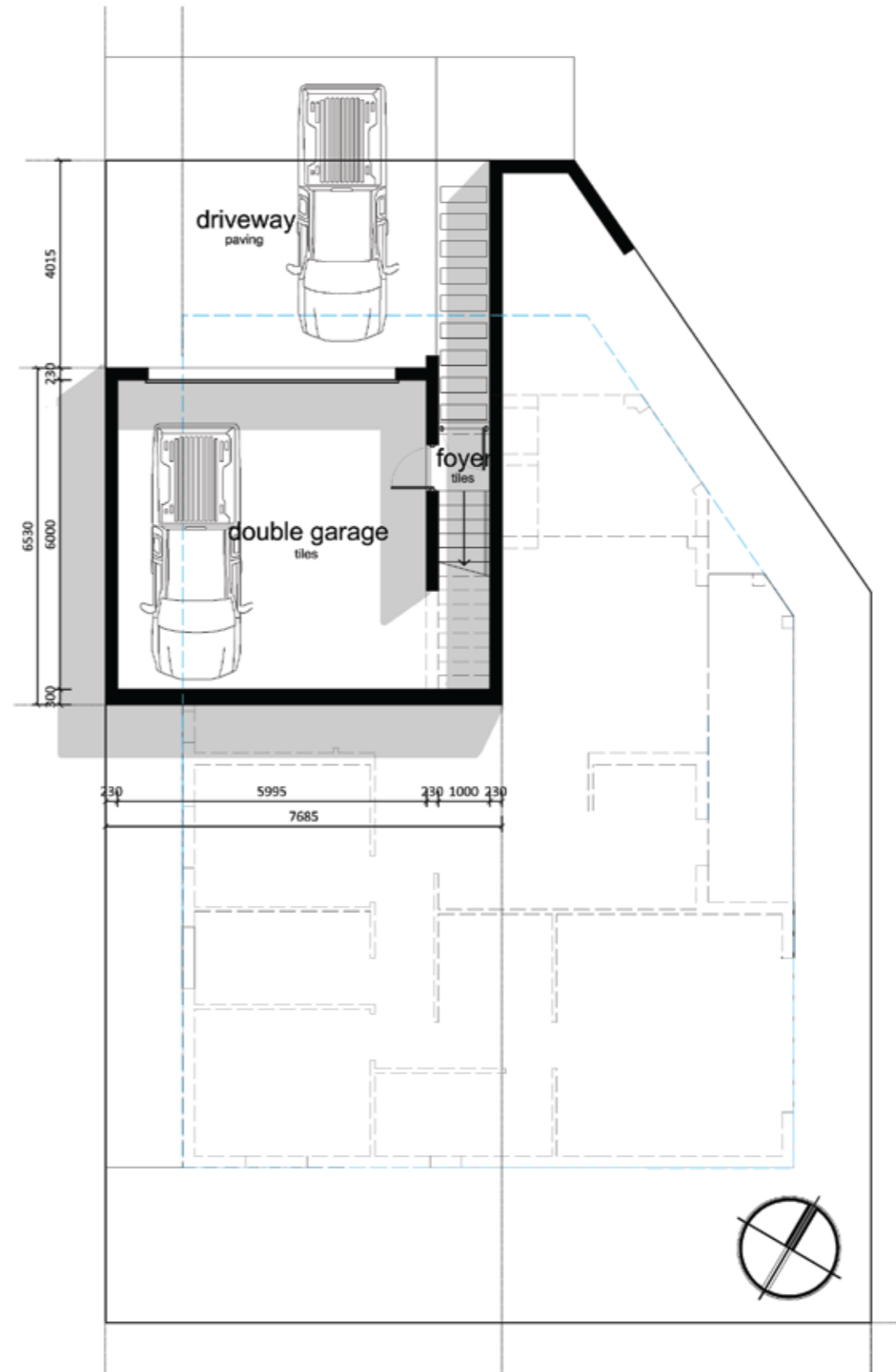
LOWER FLOOR LAYOUT
